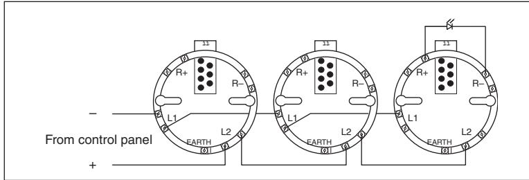
Fig 1 Wiring diagram of XP95A/Discovery loop with one remote indicator
